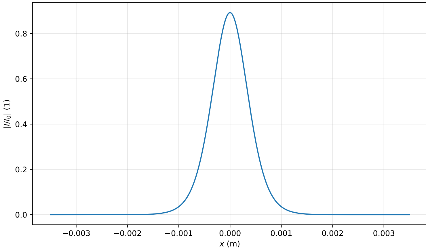
Intensity profile I(x, y = 0, z = 1.751m)/I_0 , P_{in}=0.5P_{cr} , artificial time
